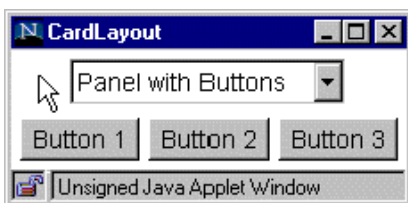
Figura 5.9. CardLayout: pantalla 1.
