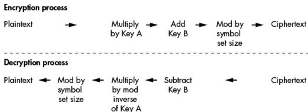
Figure 13-9: The affine cipher's encryption and decryption processes
