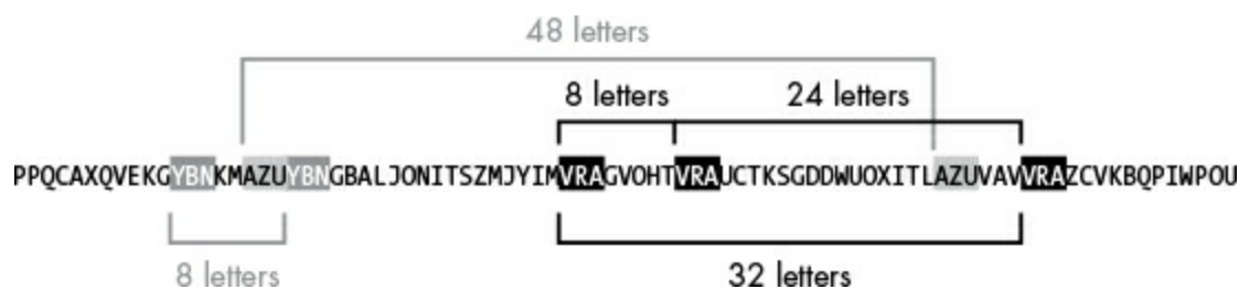
Figure 20-1: The repeated sequences in the example string
