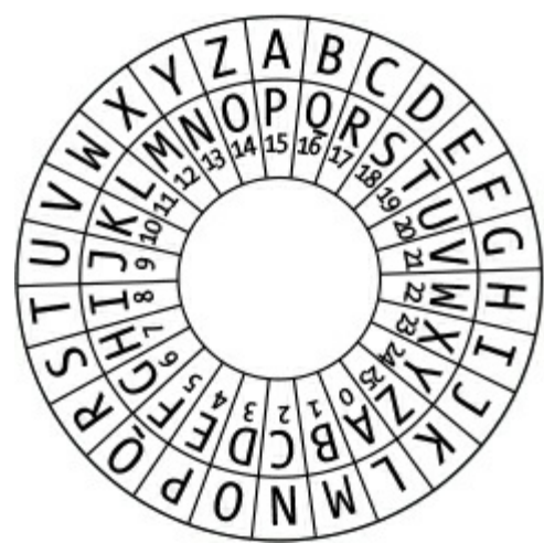
Figure 1-3: A cipher wheel set to key 15
