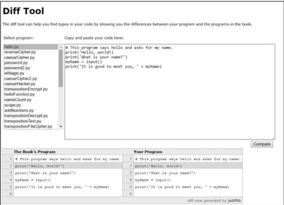
Figure 3-5: The online diff tool
