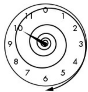
Figure 13-3: 10 o'clock + 200 hours = 6 o'clock
