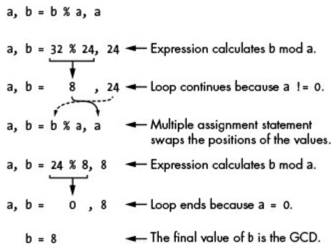
Figure 13-8: How the gcd() function works
