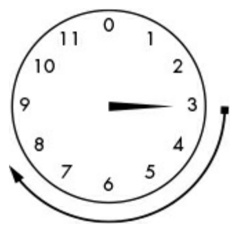
Figure 13-1: 3 o'clock + 5 hours = 8 o'clock
