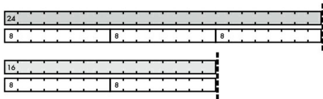
Figure 13-7: Cuisenaire rods demonstrating the GCD of 16 and 24
