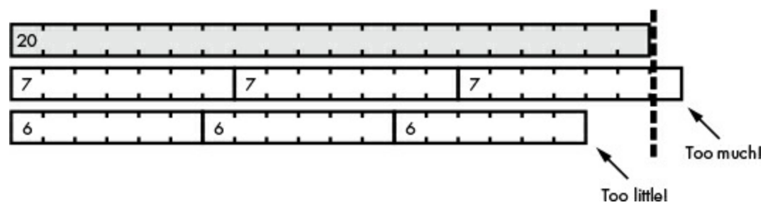
Figure 13-6: Cuisenaire rods demonstrating 6 and 7 are not factors of 20
