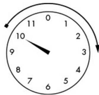
Figure 13-2: 10 o'clock + 5 hours = 3 o'clock
