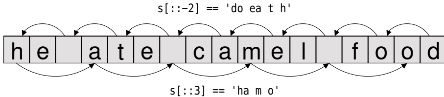
Figure 2.3 Sequence striding
