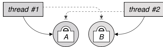
Figure 10.2 Deadlock: two or more blocked threads trying to acquire each other's locks
