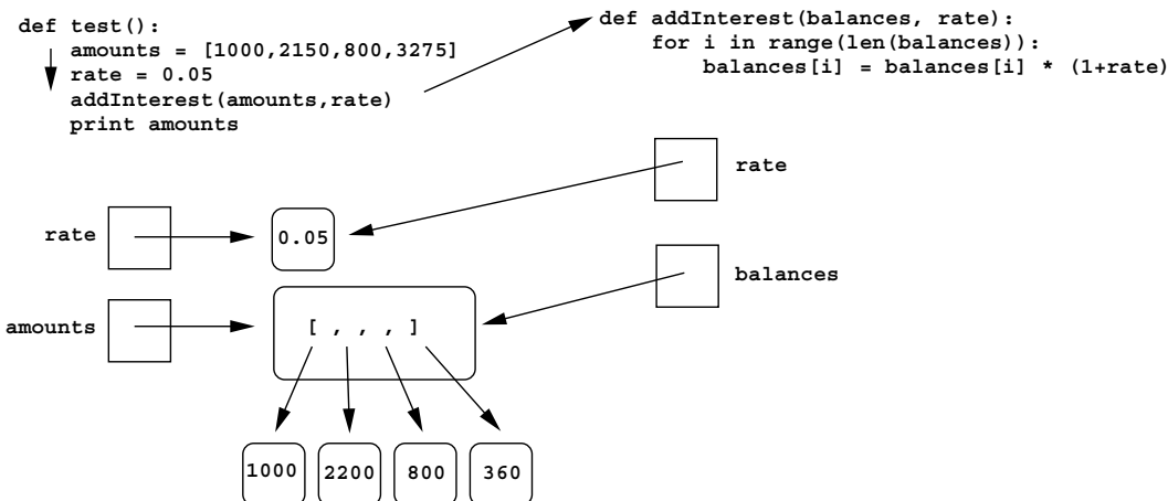
Figure 6.8: Transfer of list parameter to addInterest
