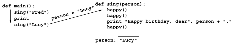
Figure 6.4: Snapshot of second call to sing .
