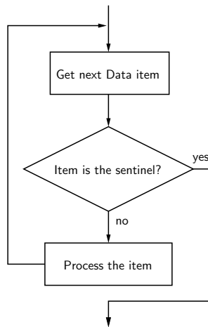
Figure 8.3: Loop-and-a-half implementation of sentinel loop pattern.
