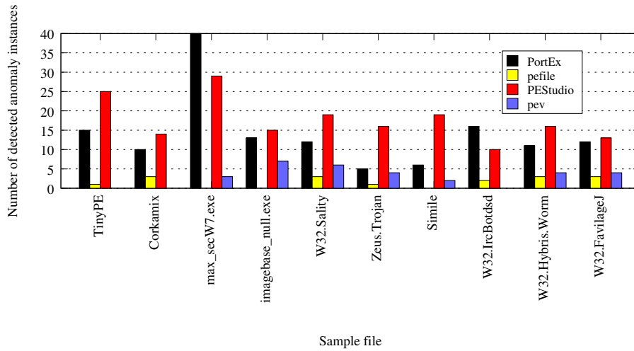
Figure 5.1: Number of detected anomalies in sample files. The value of PortEx for the file max_secW7.exe is actually 204, but the scale is cut down to 40, so the other numbers are still comparable.
