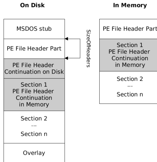
Figure 3.10: Dual PE File Header (referring to [VP11, slides 13, 14])
