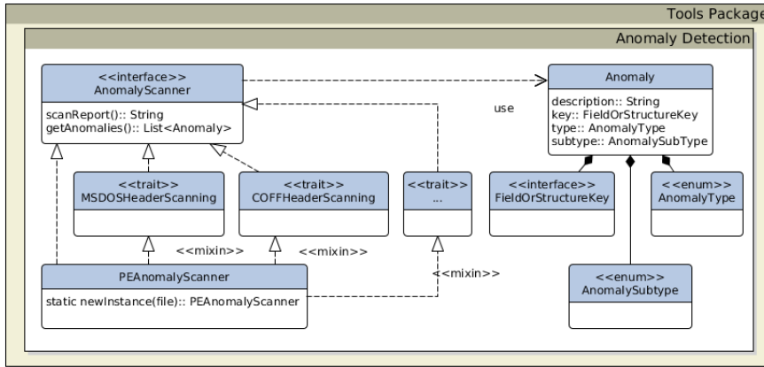
Figure 4.8: Anomaly detection package structure
