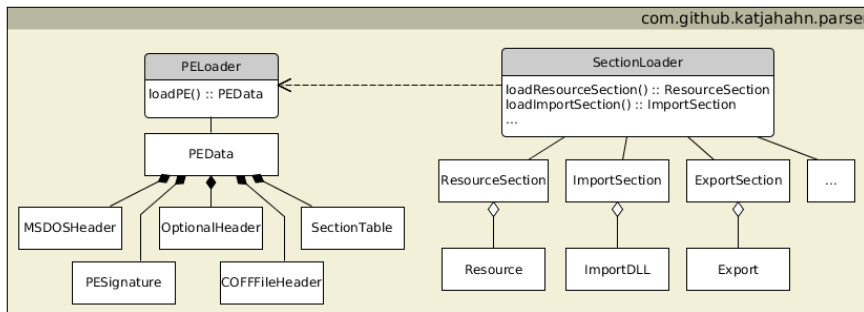
Figure 4.3: Structure of PortEx' PE format parser
