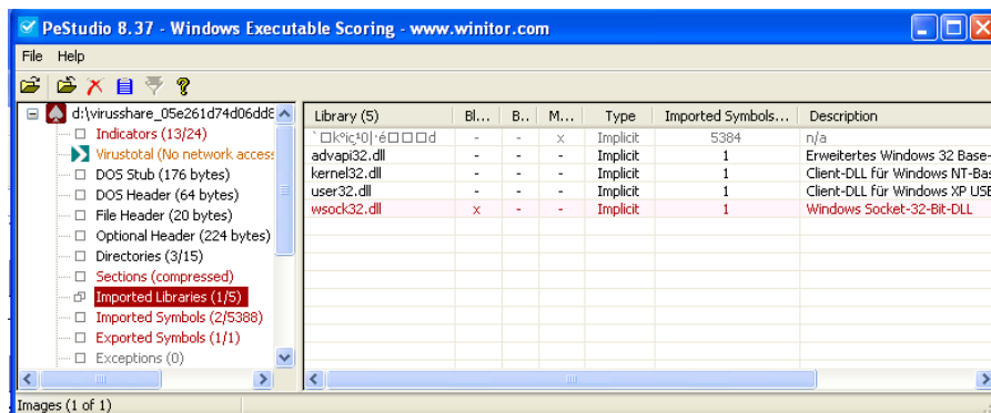
Figure 5.3: PEStudio displays a bogus import DLL with unreadable name and 5384 imported symbols for a W32.Sality infected file (#05e261d74d06dd8d35583614def3f22e), which has fractionated imports. The hidden imports are LoadLibraryA and GetProcAddress from KERNEL32.dll, which are indicators for a packed file.
