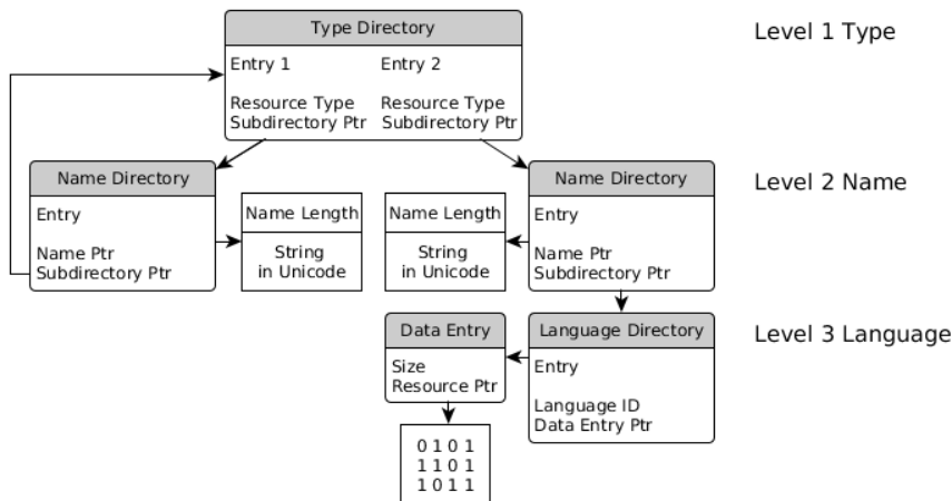
Figure 3.9: Resource tree with a loop
