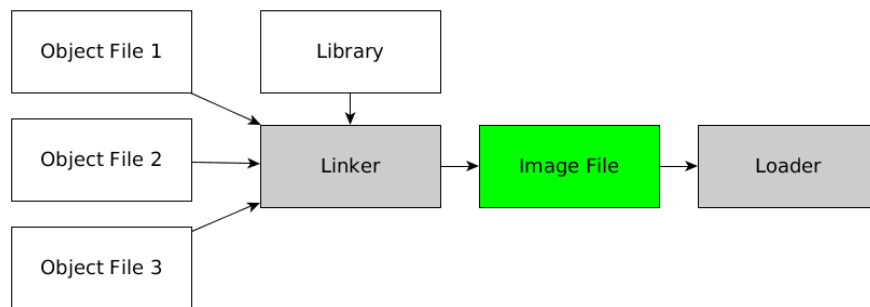
Figure 3.1: The linker combines object files and libraries to an image file, which is used as input by the loader
