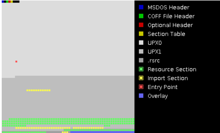
Figure 3.6: Fractionated imports (yellow) and resources (green), output by PortEx, malware sample #7dfcbb865a4a5637efd97a2d021eb4b3
