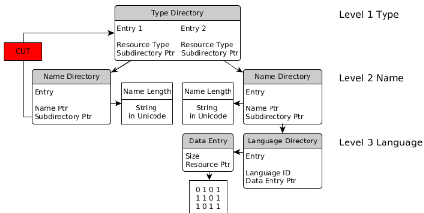
Figure 4.5: A loop in a resource tree is cut by the PortEx parser
