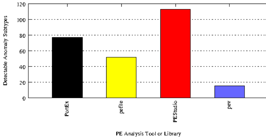
Figure 5.2: Number of detectable anomaly subtypes
