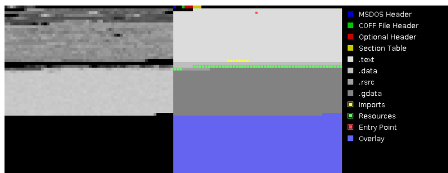
Figure 4.11: PE visualiser, example output for a PE file infected with W32.Sality ; the left side shows the local entropy, the right side the structure of the file.
