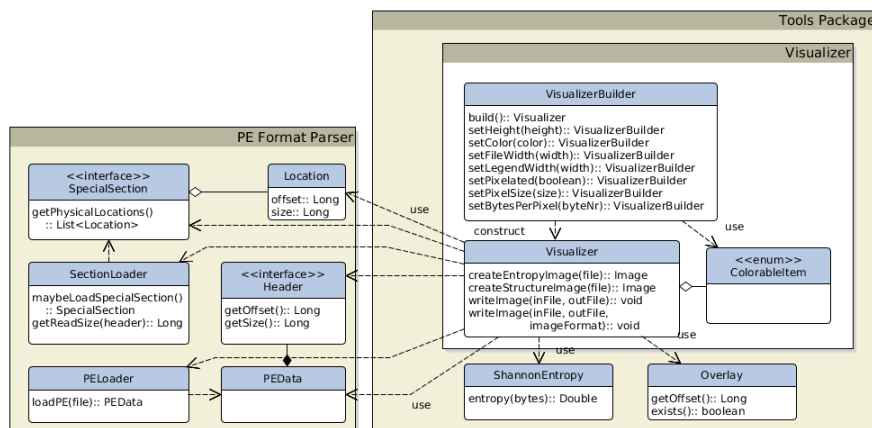
Figure 4.10: Visualiser package structure and dependencies
