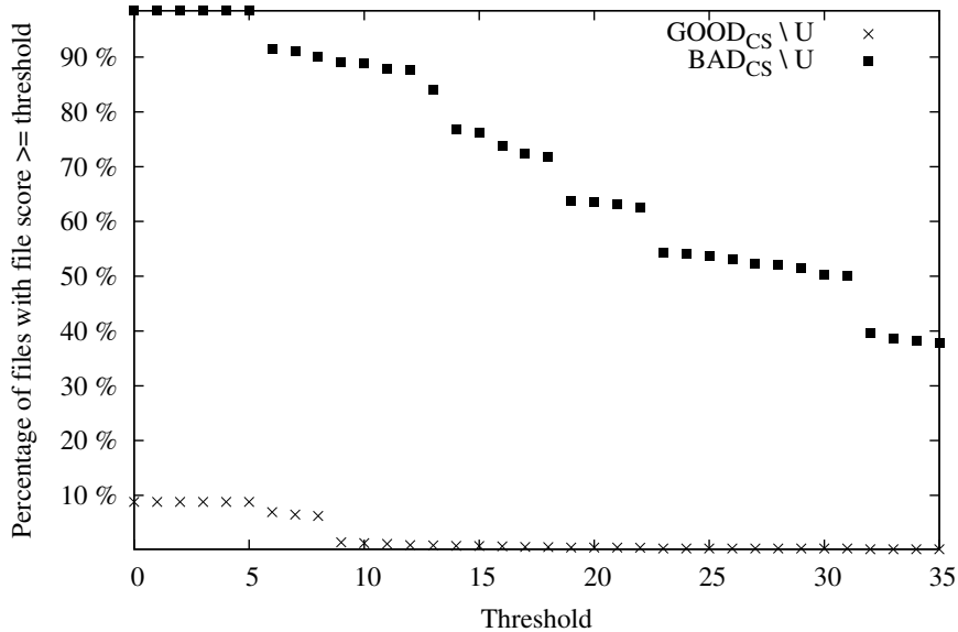
Figure 5.7: Percentage of files whose file score is greater than or equal to a given threshold using the selective scanner
