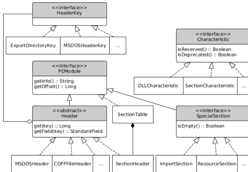
Figure 4.4: PE parser interfaces of PortEx
