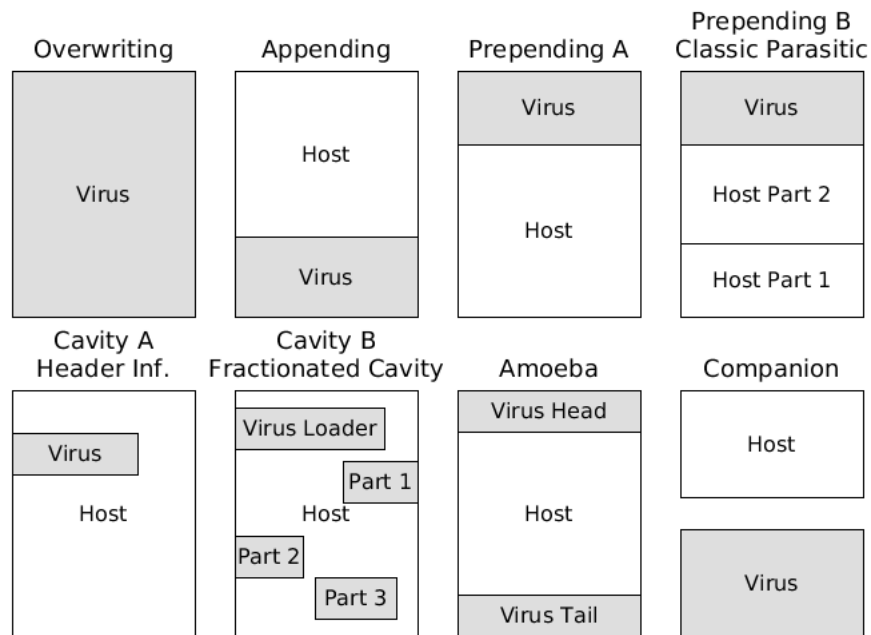
Figure 2.3: File infection strategies
