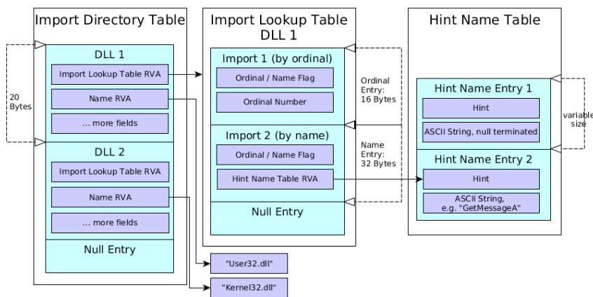
Figure 3.4: Typical Import Section layout
