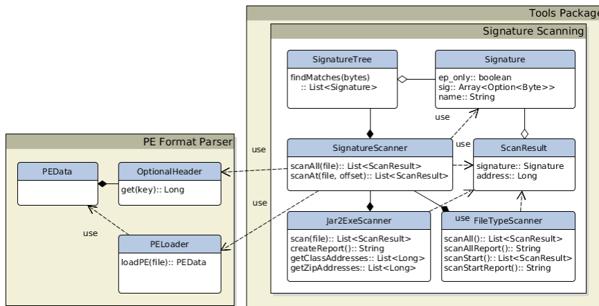
Figure 4.7: Signature scanning package structure and dependencies
