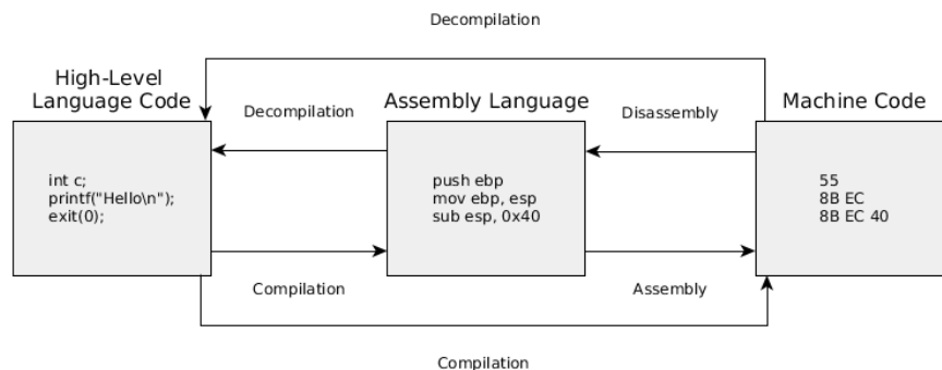
Figure 2.4: Compilation, assembly, and reversing processes; referring to [SH12, p. 67]
