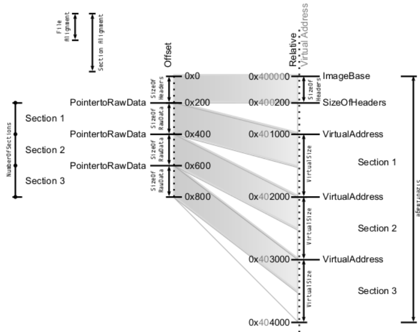
Figure 3.5: Mapping a PE file from disk (left side) to memory (right side) by [Alb13].
