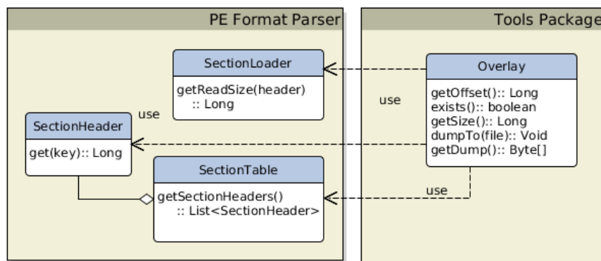
Figure 4.9: Overlay tool structure and dependencies
