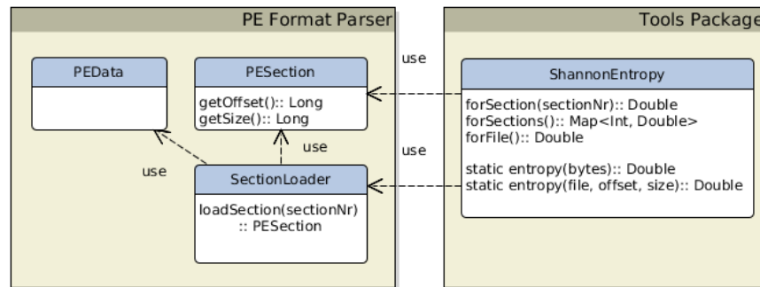
Figure 4.6: Entropy tool and dependencies
