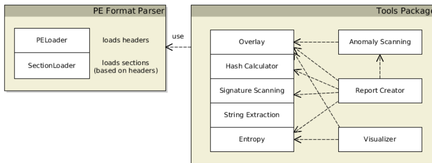
Figure 4.2: Main structure of PortEx and dependencies of the modules
