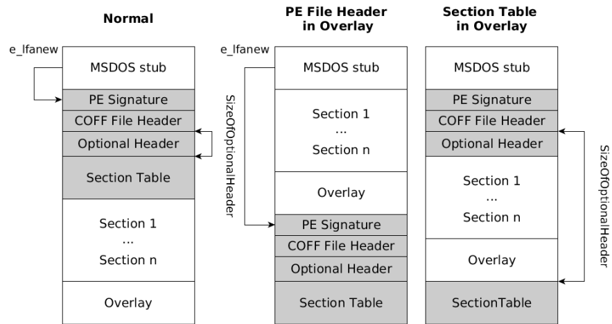
Figure 3.8: The PE File Header (grey) and the Section Table can be placed in overlay (referring to [VP11, slides 13, 14])
