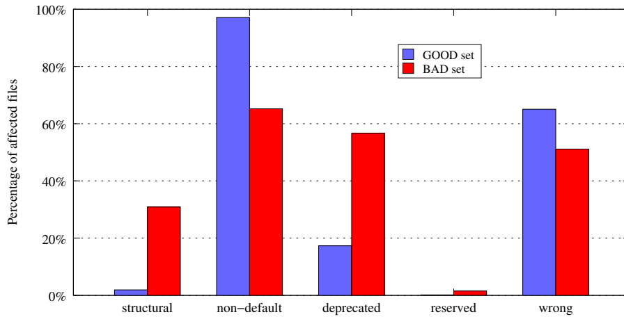
Figure 5.4: PE files with at least one anomaly of specified type
