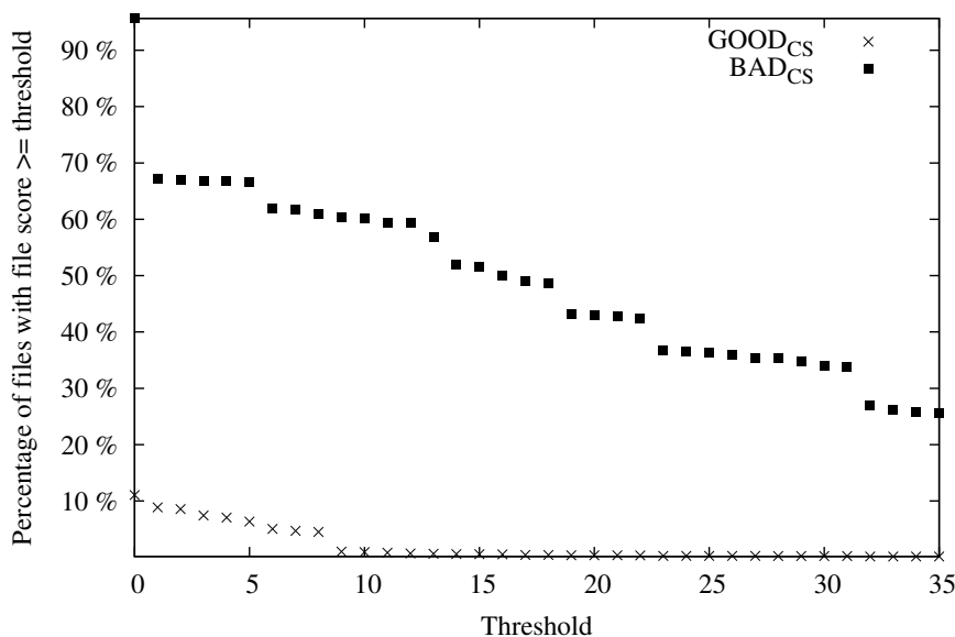
Figure 5.6: Percentage of files whose file score is greater than or equal to a given threshold using the unselective scanner
