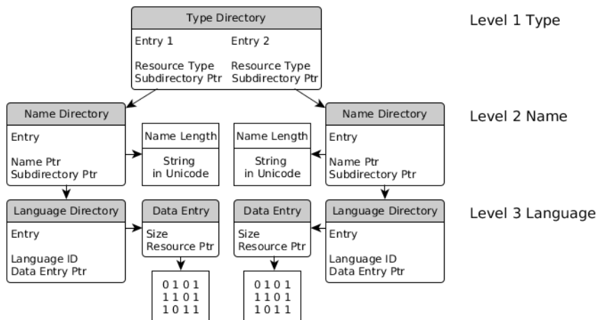
Figure 3.3: Resource tree with two resources, referring to [Kat13]
