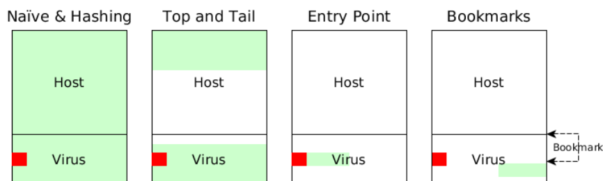
Figure 2.5: The scanned area (green) of an infected file with different string scanning strategies applied. The red rectangle marks the entry point. The virus example is an appending file infector that modifies the entry point of the host file to point to the virus body.
