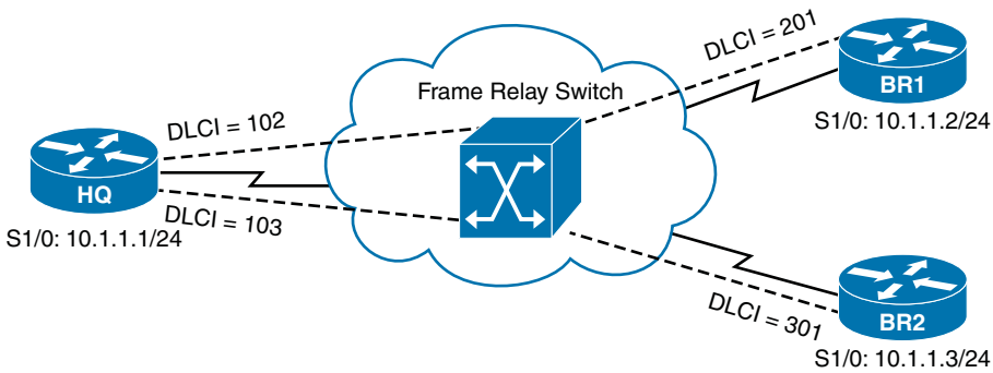
Figure 1-14 NBMA Network Type
