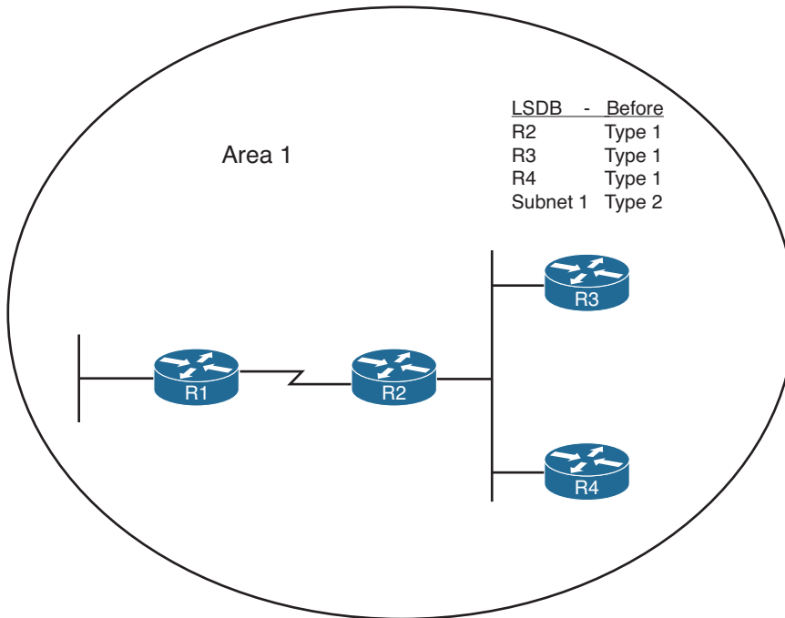
Figure 8-10 Flooding Throughout an Area
