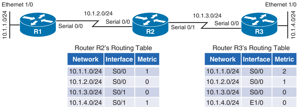
Figure 1-5 Routing Loop: Before Link Failure
