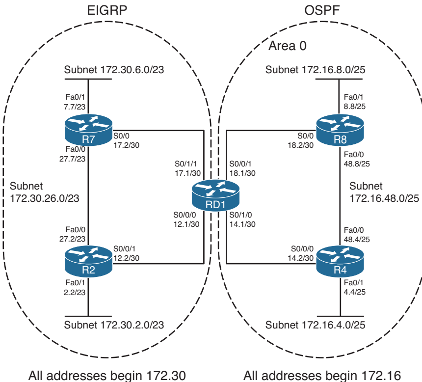
Figure 10-6 Sample Internetwork Used for Redistribution Examples
