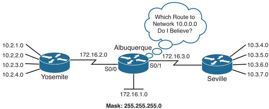
Figure 5-21 Discontiguous Network 10.0.0.0
