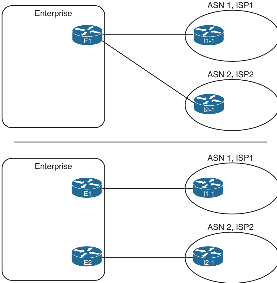
Figure 13-13 Single-Multihomed Designs
