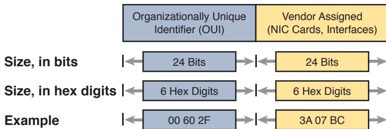
Figure 2-15 Structure of Unicast Ethernet Addresses
