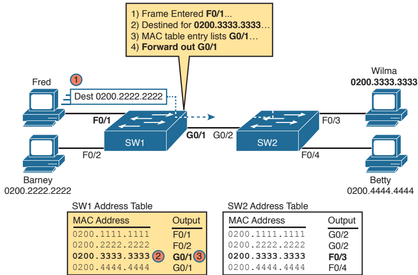
Figure 7-4 Forwarding Decision with Two Switches: First Switch
