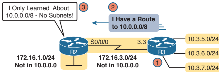
Figure 19-12 Autosummarization Example
