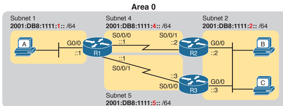
Figure Q-12 Single-Area Design in OSPFv3 Configuration Example
