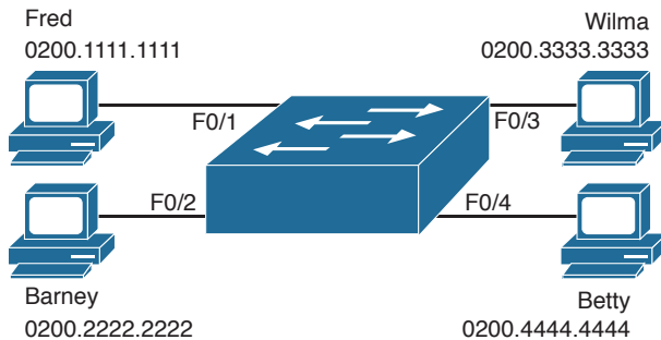
Figure 7-9 Single Switch Topology Used in Verification Section
