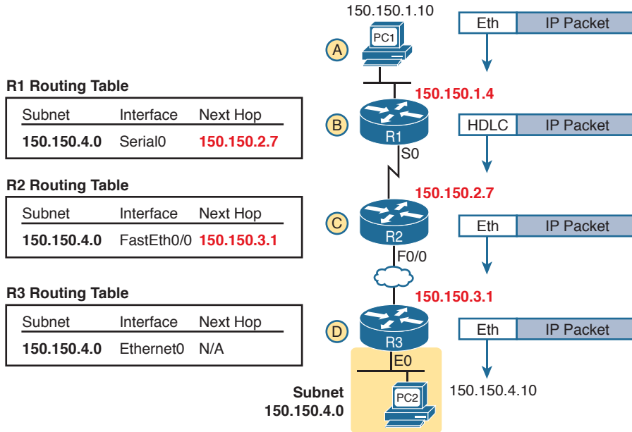
Figure 4-11 Simple Routing Example, with IP Subnets
