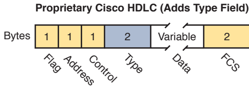
Figure 3-6 HDLC Framing
