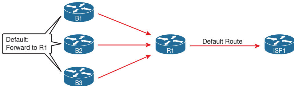
Figure Q-5 Default Routes Resulting from the default-information originate Command
