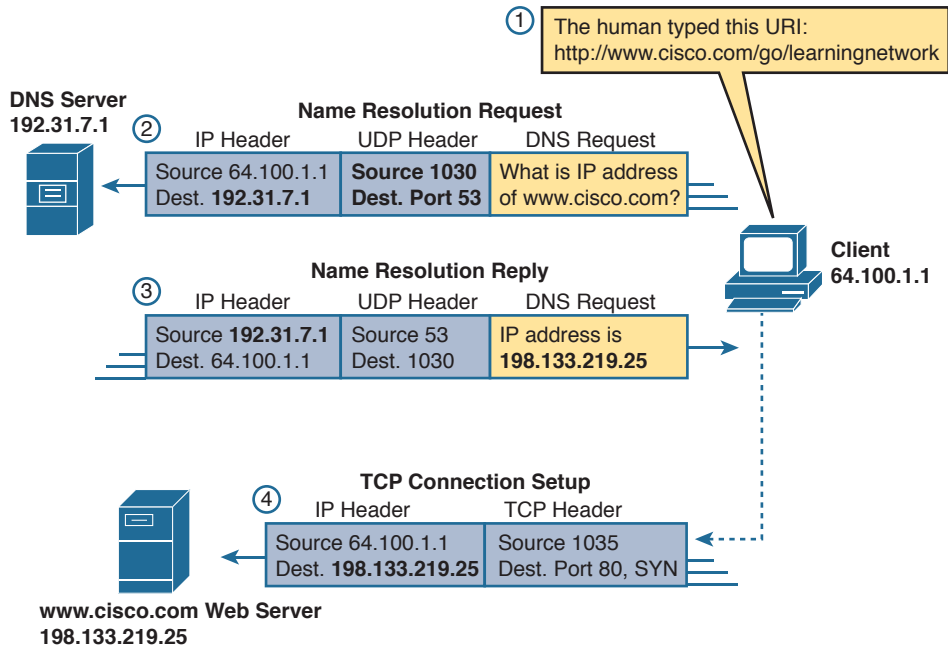
Figure 5-12 DNS Resolution and Requesting a Web Page
