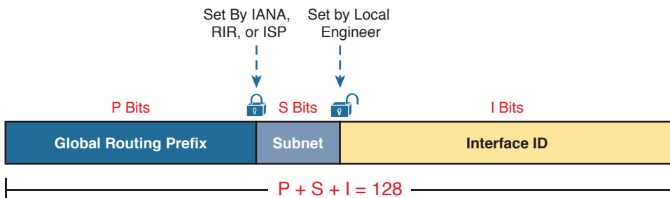
Figure 29-9 Structure of Subnetted IPv6 Global Unicast Addresses
