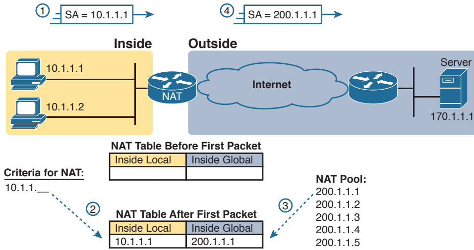
Figure 27-5 Dynamic NAT
