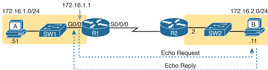
Figure 24-8 IP Helper Address Effect
