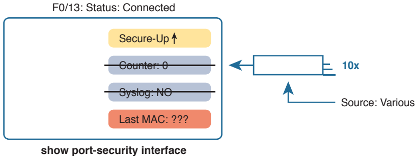
Figure 12-7 Summary of Actions: Port Security Violation Mode Protect
