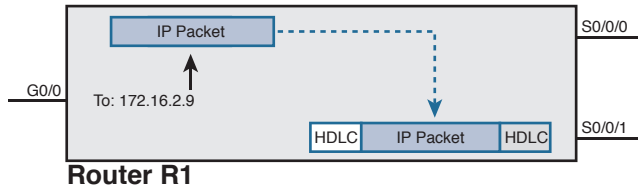
Figure 18-8 Routing Step 4 on Router R1: Encapsulating the Packet
