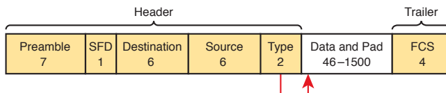
Figure 7-2 IEEE 802.3 Ethernet Frame (One Variation)
