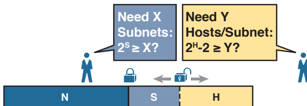
Figure 13-15 Borrowing Enough Subnet and Host Bits
