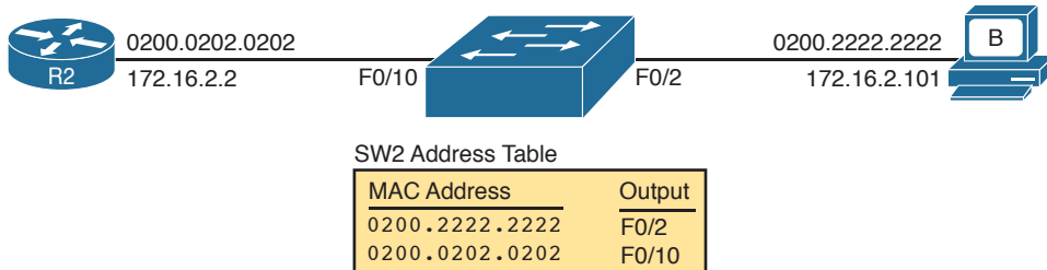
Figure 23-5 Router and Host ARP Tables, with the Switch MAC Address Table
