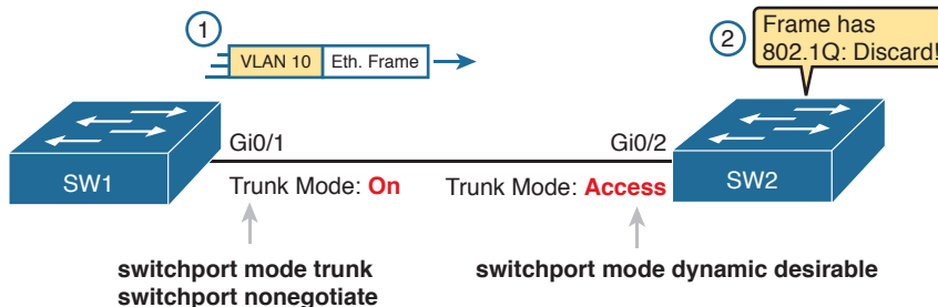
Figure 12-9 Mismatched Trunking Operational States
