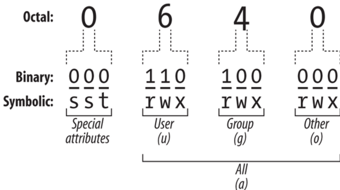
Figure A-2. File Permission Bits
