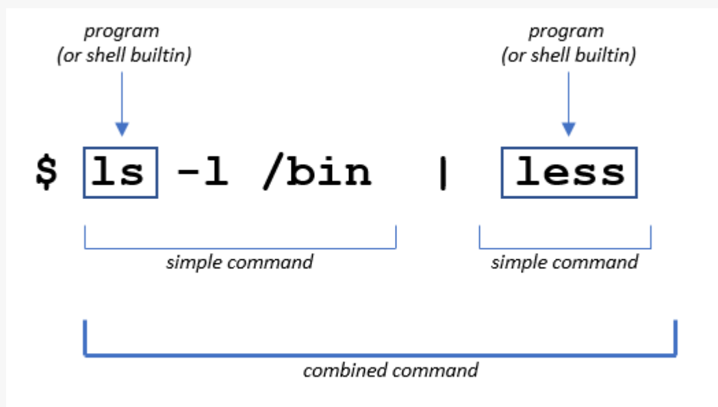
Figure 1-1. Programs, simple commands, and combined commands are all referred to as “commands”
