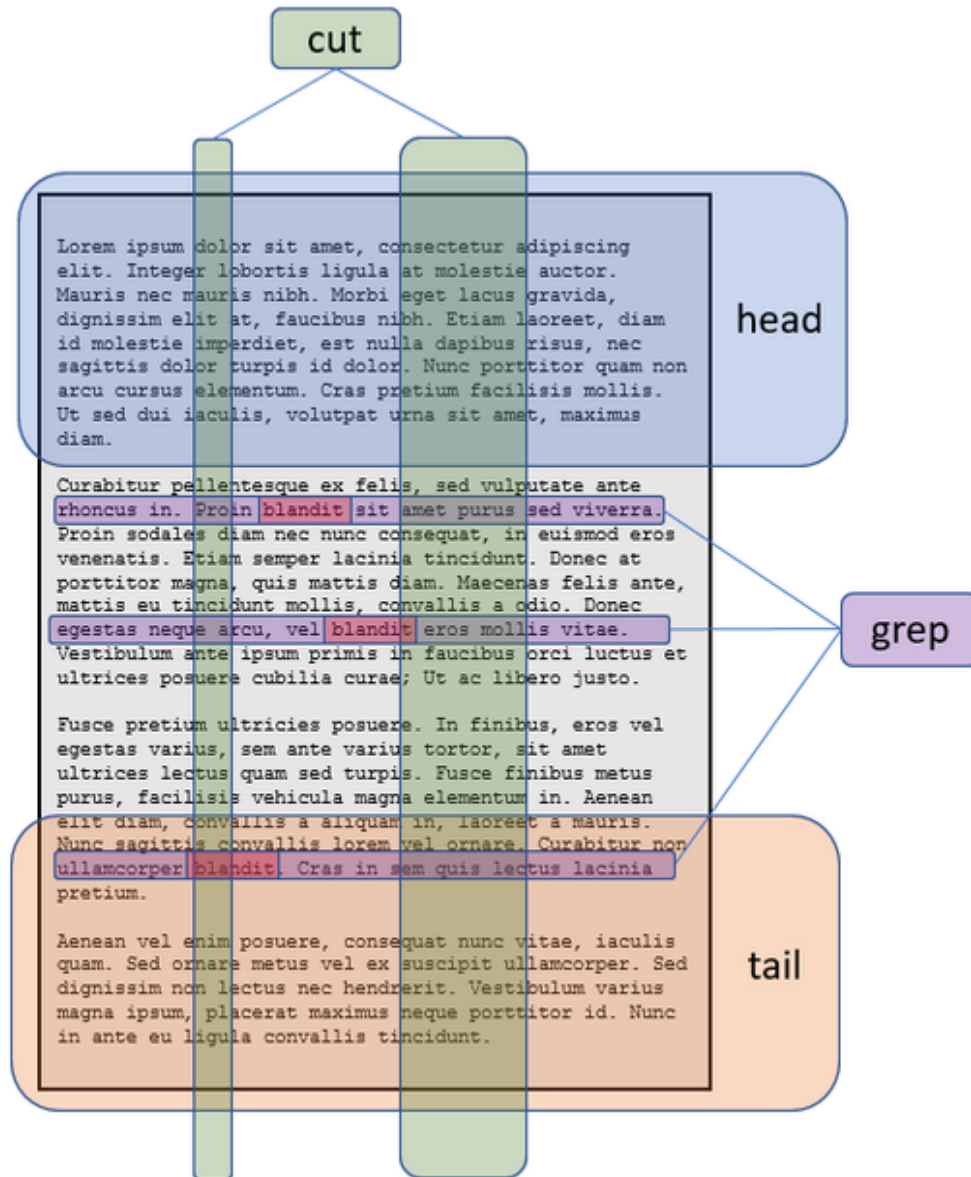
Figure 5-1. head , grep , and tail extract lines, and cut extracts columns. In this example, grep matches lines containing the string "blandit."
