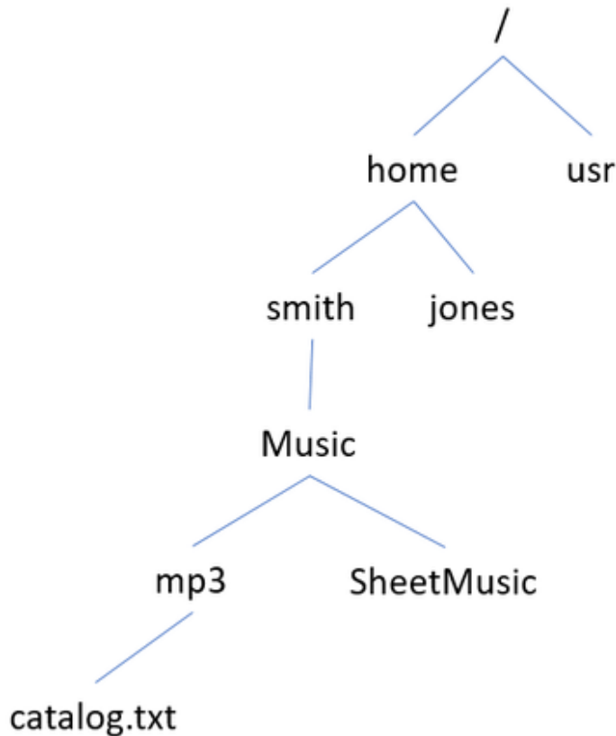
Figure A-1. Paths in a Linux Directory Tree
