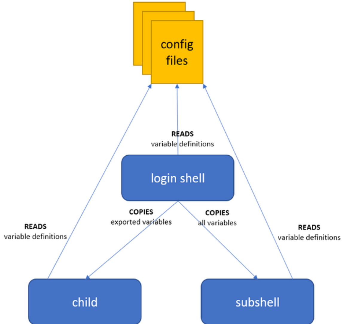
Figure 6-1. Shells may share variables and values by export or by reading the same configuration files
